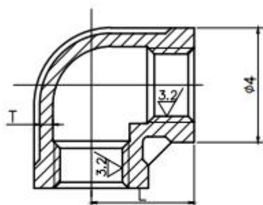
90° Elbow
