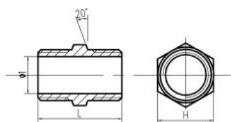
Hex Nipple
