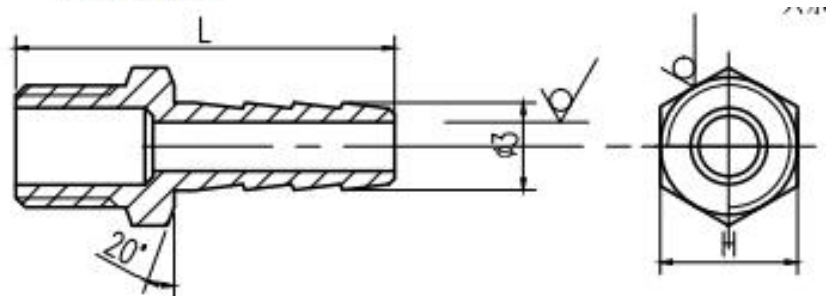
Hose Nipple
